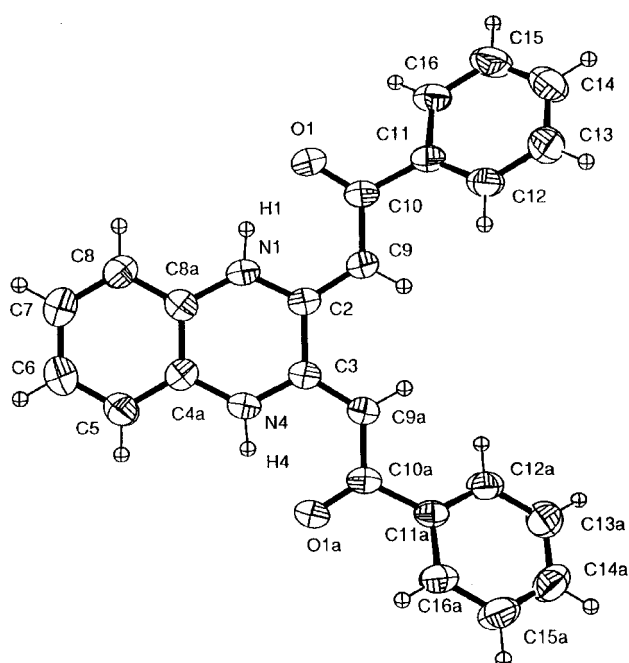
Fig. 1 ORTEP drawing of compound 3.
