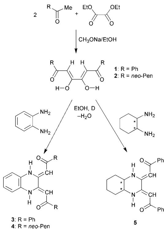
Scheme 2 Synthesis of the quinoxaline-like derivatives 3–5
