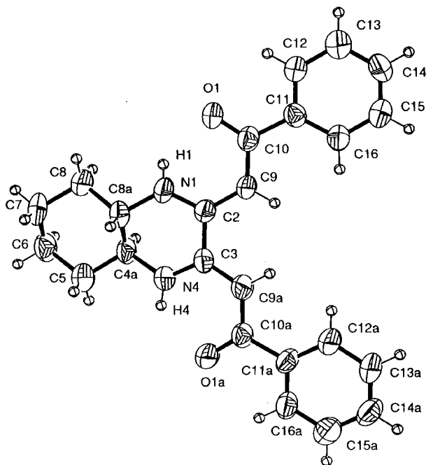
Fig. 3 ORTEP drawing of compound 5.
