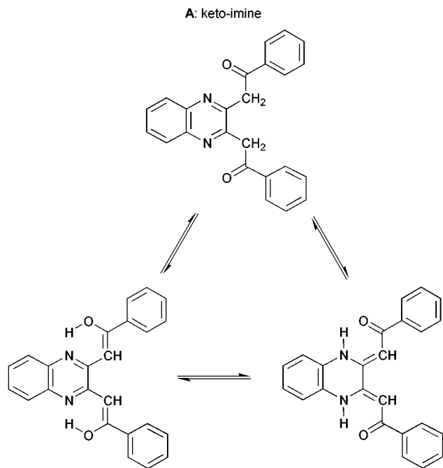
Scheme 1 Different tautomeric forms of quinoxaline derivatives.
