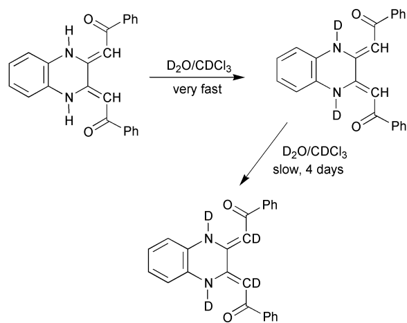
Scheme 3 H/D exchange reaction.
