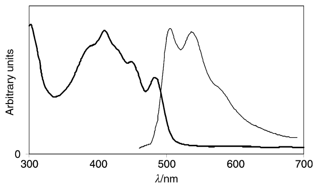
Fig. 2 UV-vis (bold line) and fluorescence spectra of compound 3 .
